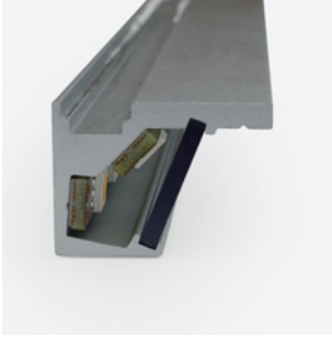
5° & 45° LED position TANA R014 (x2) only
